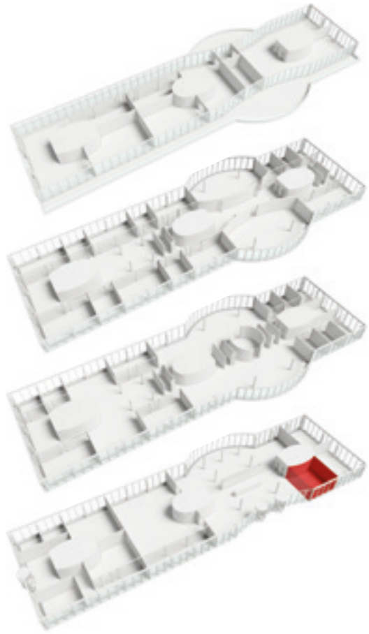
WARTEN / WAITING
