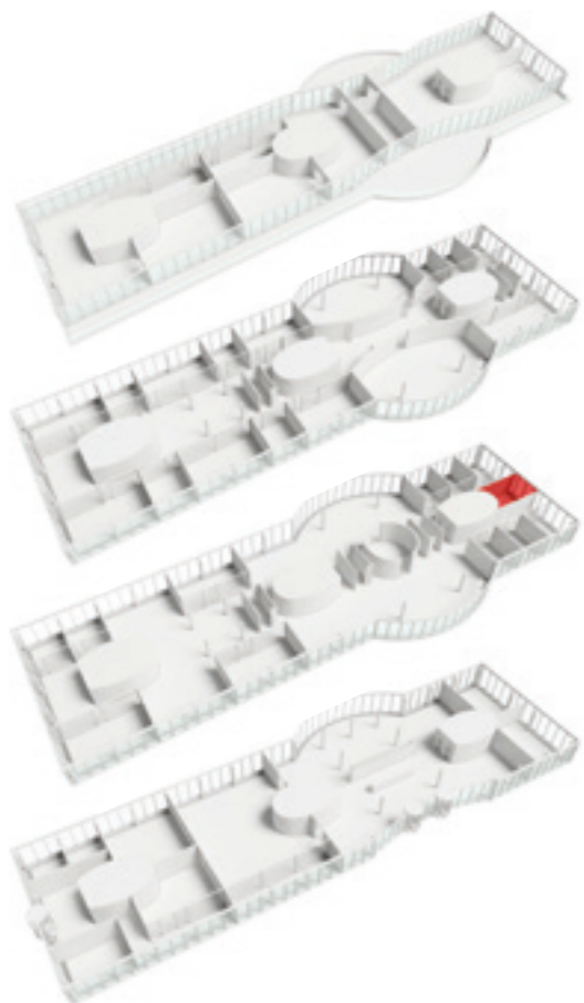
DIALOG / TALK
