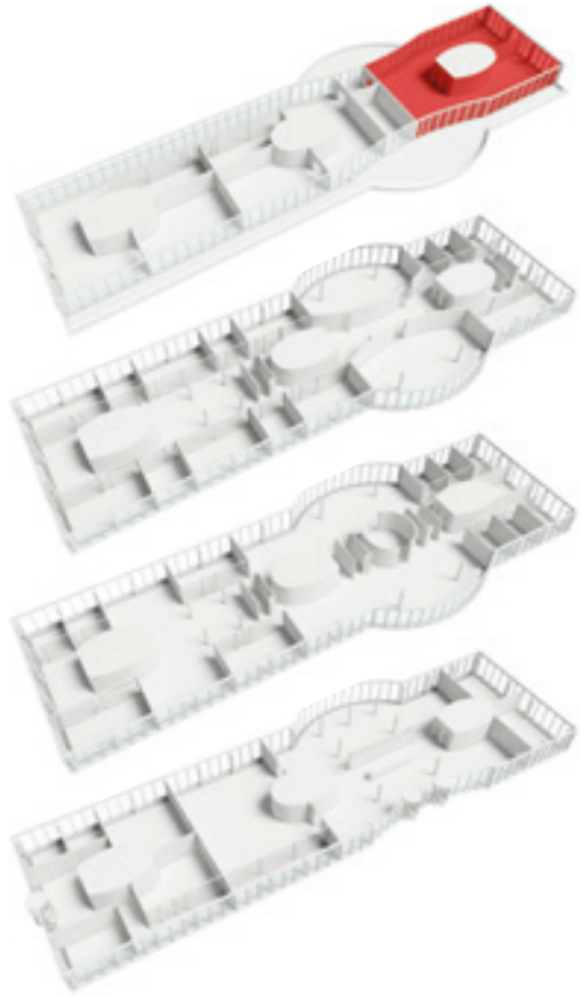
MANAGER / MANAGER
